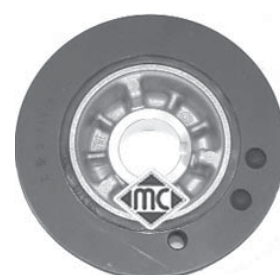
4485 Ø 127 mm - 6 canales PSA motor XU7 (1.8)-XU10 (2.0) 306-405-Jumpy-406-Xantia r.o. 0515.H6
