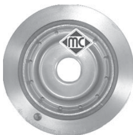
4465 Ø 133 mm - 6 canales motores K4J 1.4/16v y K4M 1.6/16v Clio-II - Kangoo - Megane - Laguna-II r.o. 8200313231-8200544135-8200392683
