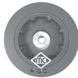
2849 Ø 132 mm - 6 canales motor 1.9Diesel F8Q Megane-Express-19-Clio-Kangoo r.o. 7700112499-8200386445
